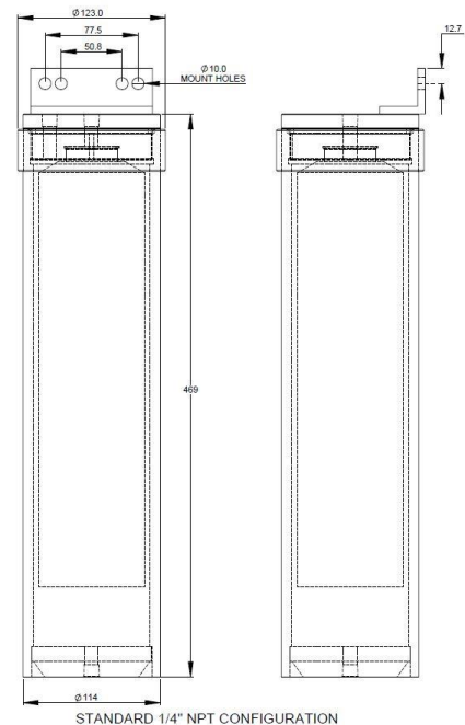
STANDARD 1/4" NPT CONFIGURATION
