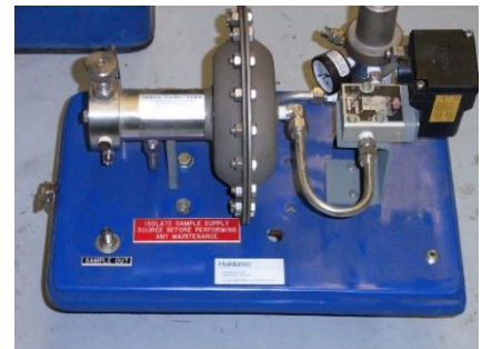
A grab sampler mounted in a GRP enclosure for Condensate
